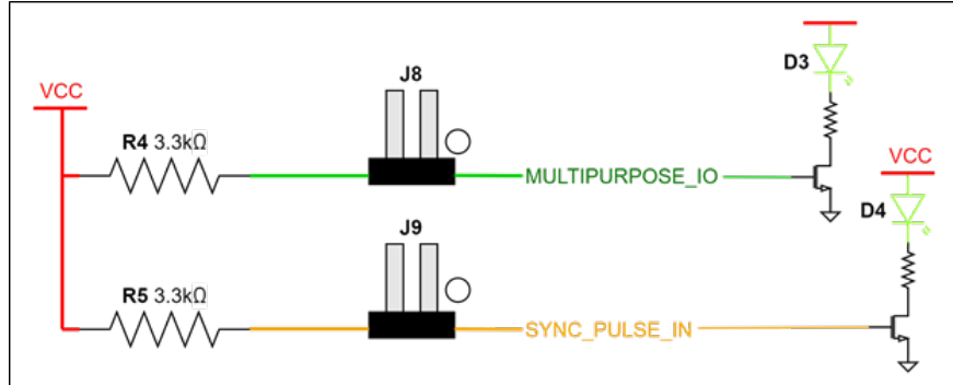
Figure 7.3: J8 & J9 Circuitry
