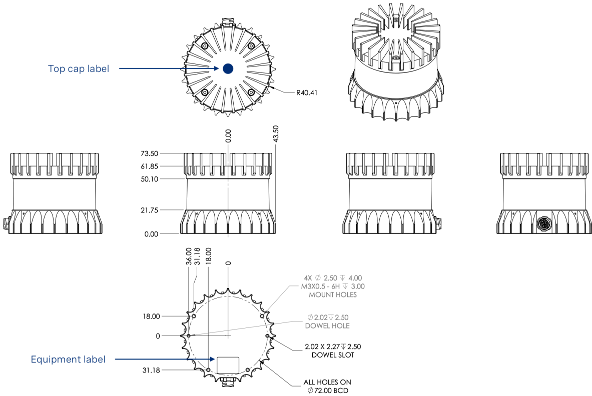
Figure 3.1: Sensor Components
