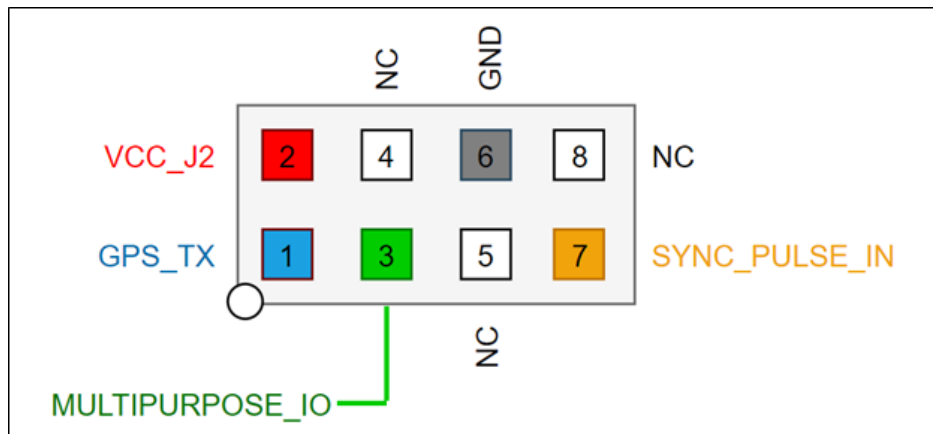
Figure 8.2: J7 Circuitry
